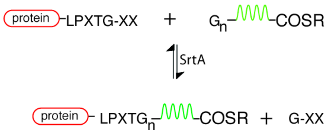
Scheme 1. Protein \alpha thioester synthesis using SrtA
