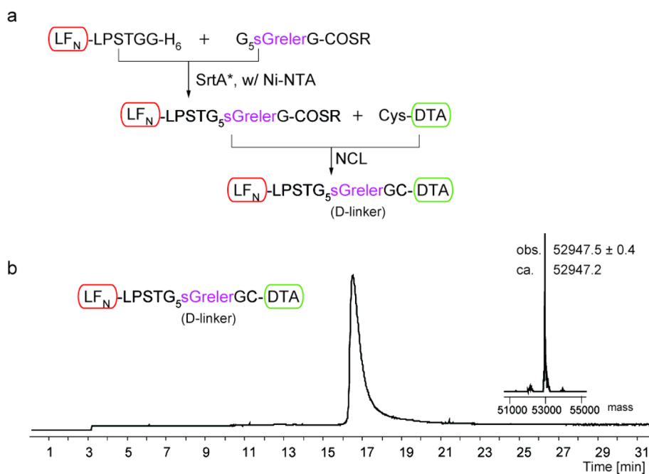
Figure 3. Installing a D-peptide segment between \text{LF}_N and DTA. (a) Synthetic strategy used to modify the linker region (lower case = D-amino acid). (b) LCMS and deconvoluted MS (inset) for \text{LF}_N -D-linker-DTA. The reaction conditions are reported in the supporting information. LCMS traces are shown as total ion current.
