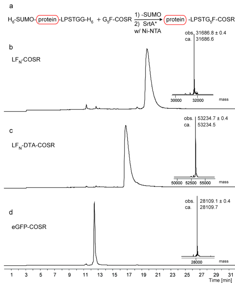
Figure 2. LCMS data for protein α thioester synthesis using SrtA*. (a) SML of model proteins. (b)–(d) LCMS and deconvoluted MS (inset) of the main component for LF N , LF N -DTA and eGFP thioesters. Reaction conditions: (1) SUMO cleavage: 1 μg SUMO protease per 1 mg protein for 90 min at room temperature. (2) SML: 500 μM G 5 F-COSR, 100 μM protein-LPSTGG, 5 μM SrtA*, 75 μl Ni-NTA agarose slurry per mg protein, SrtA* buffer, pH 7.0, 30 min. LCMS traces are shown as total ion current.
